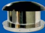
Roof Extractor Fan Size : Ø280mm - Ø 400mm Air Flow : 500-4200 CMH
