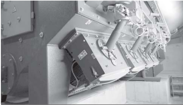
The eight Gamma 400G high-performance turbines with “Y” shaped throwing blade guarantee consistent high-quality shot blasting results.
